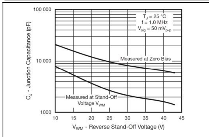
Figure 6 - Typical Junction Capacitance
